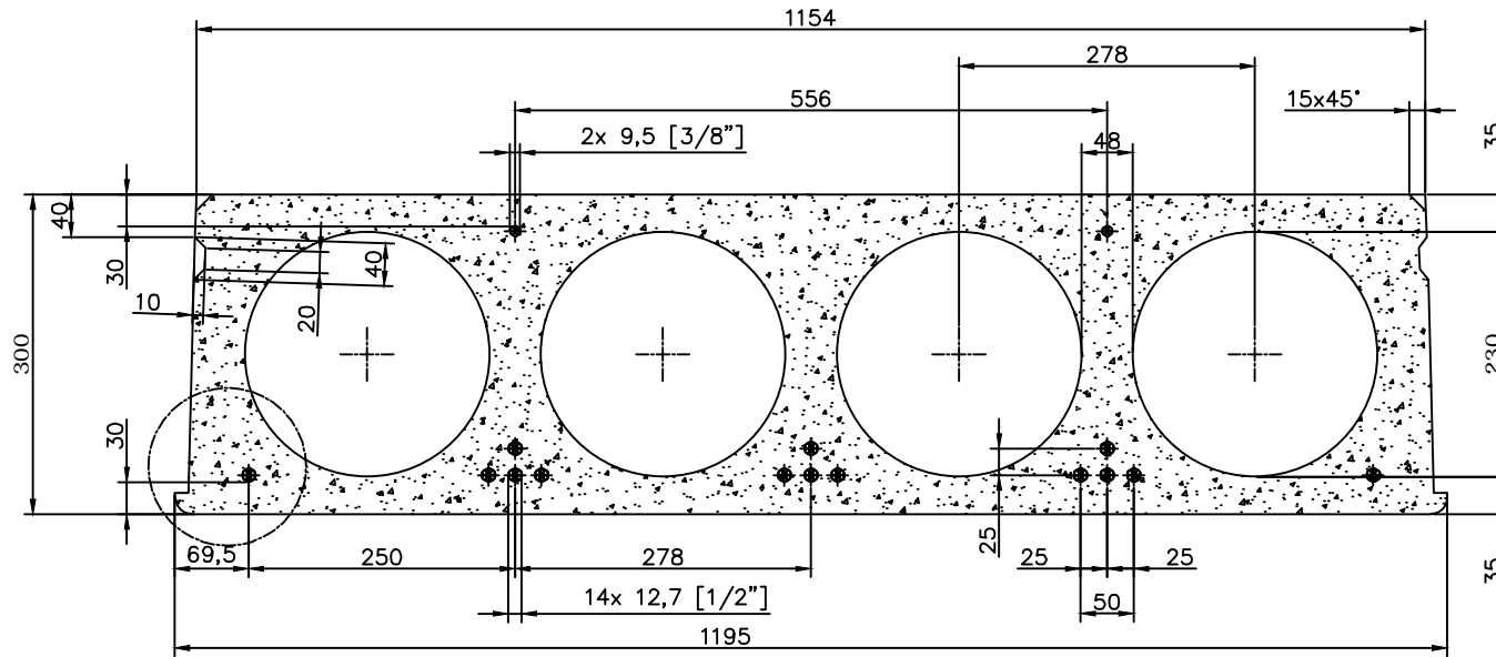
Concrete Slab shown with maximum wire layers
